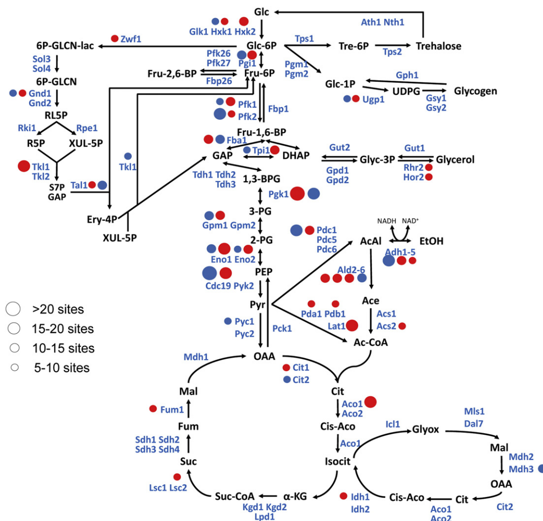
Fig. 3. Acetylated (red circles) and ubiquitinated (blue circles) enzymes mapped on the central carbon metabolism scheme. Circle size represents the number of modified sites. Only enzymes modified on more than 5 lysines are marked. The map was generated querying CPLM database [46,47].
