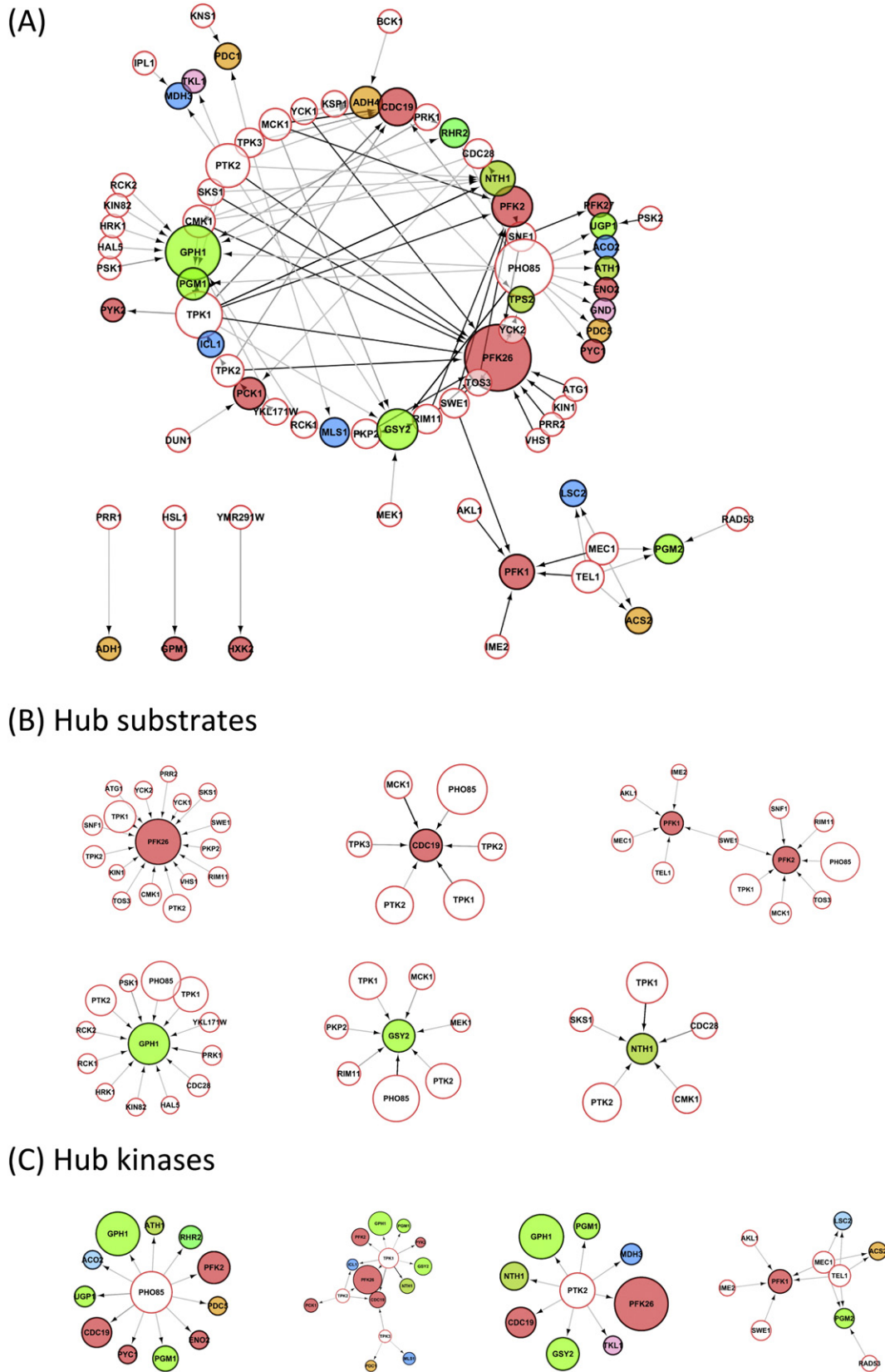
Fig. 2. (A) Phosphorylation network of the central carbon metabolism enzymes. The network reports the known target–kinase associations. Red bordered nodes indicate a kinase, filled nodes indicate a substrate. Red nodes indicate glycolytic enzymes, different shades of green indicate enzymes of glycolysis-branching pathways (trehalose, glycogen and glycerol biosynthesis), pink nodes indicate pentose phosphate enzymes, orange nodes indicate fermentation enzymes and blue nodes indicate TCA/glyoxylate cycle enzymes. Node size represents the degree of connection. The network was generated querying the Yeast Kinase Interaction Database (KID, http://www.moseslab.csb.utoronto.ca/KID/ ; [31]; updated 2014-01-10) with the full list of enzymes of the central carbon metabolism pathways. Data visualization and analysis were performed with Cytoscape [94]. (B–C) Sub-networks of the most connected substrates (B) and kinases (C), extracted from the network in (A).
